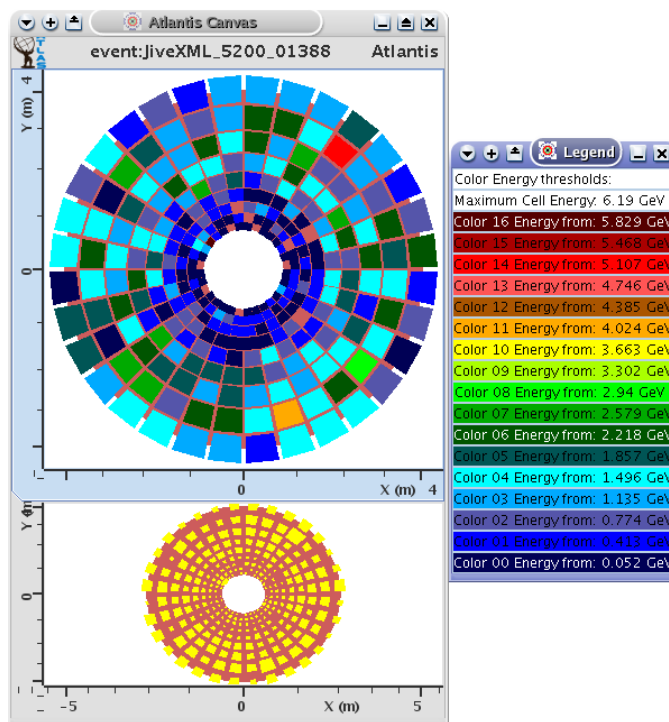
Figure 4.10: The colour-by-energy option makes it easier to find an energetic cell, here in the summed end-cap. The legend can also be used to see the scaling of the colours.
