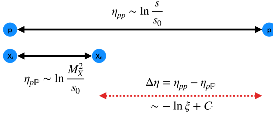
Figure 2.2: The rapidity gap formed by a pX system with \eta shown on the x -axis.
