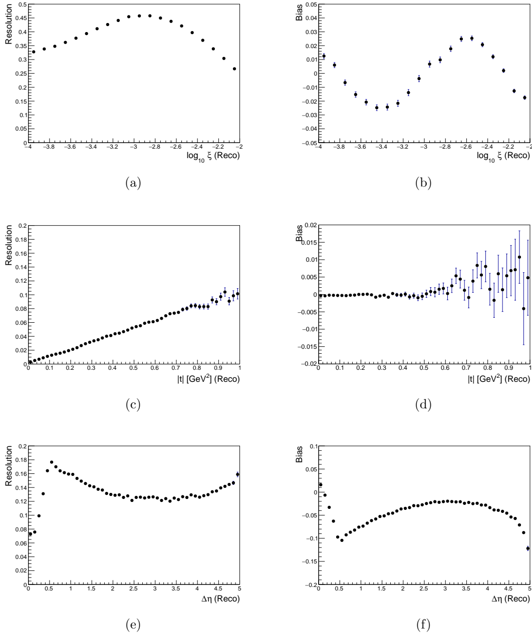
Figure 4.14: The bias and resolution as a function each reconstructed variable. For |t| and \log_{10} \xi this is shown following the calibration.
