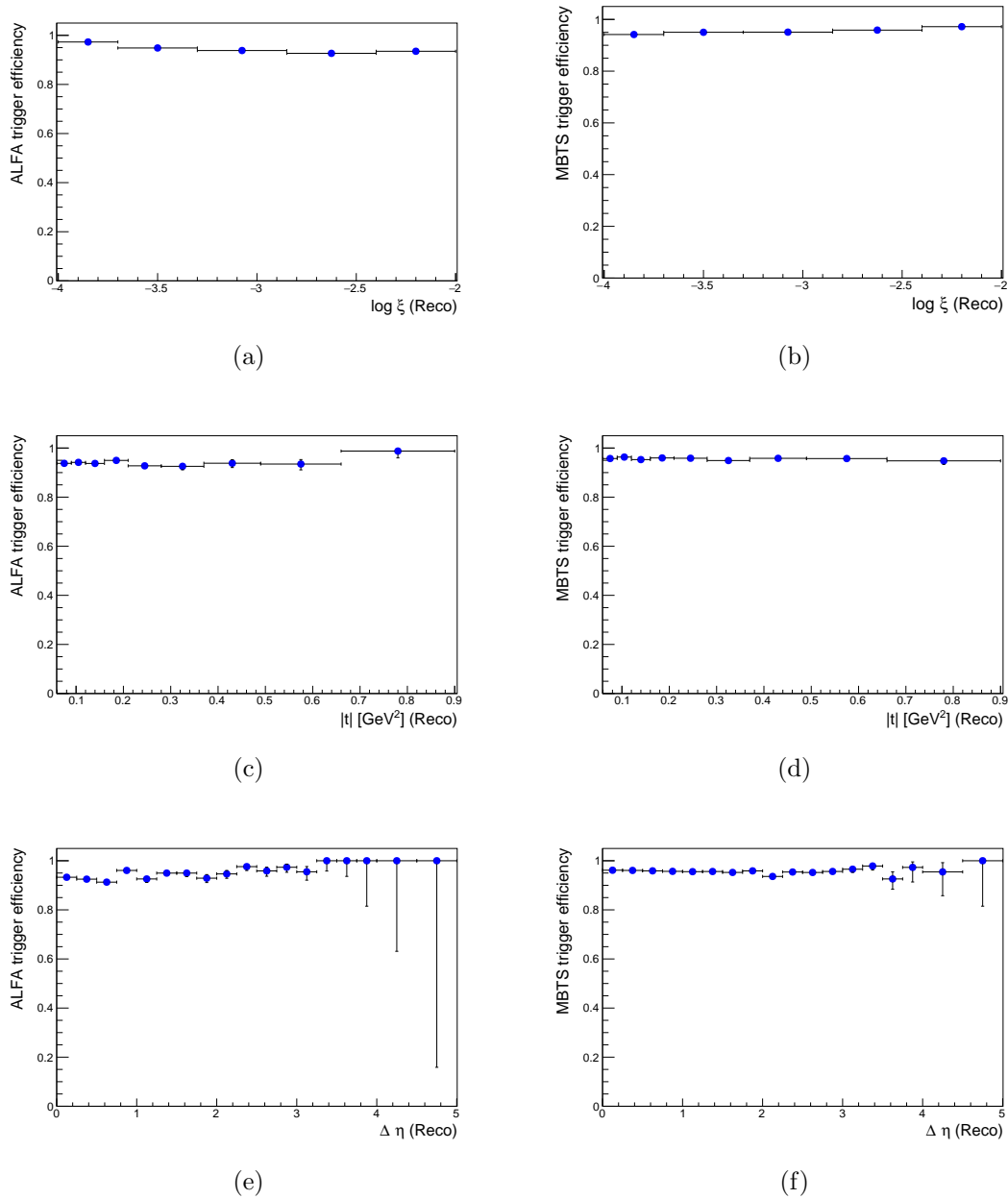
Figure 5.4: The calculated trigger efficiency as a function of each of the analysis variables. The efficiency is calculated separately for the ALFA and MBTS components of the trigger.
