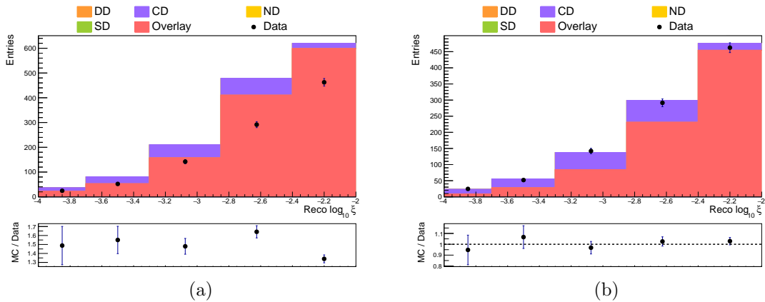
Figure 6.3: Reconstructed distributions of \log_{10} \xi in the two proton control region, before (a) and after (b) re-weighting using equation 6.2.
