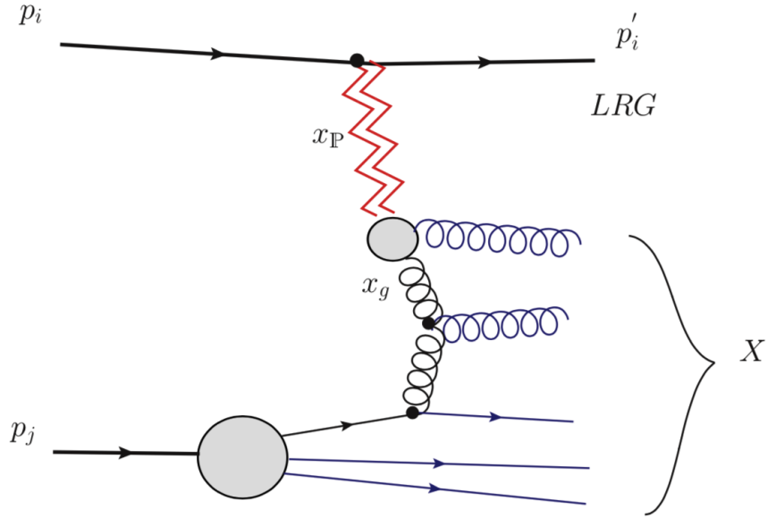
Figure 2.12: A Feynman diagram showing the method that PYTHIA follows for modelling SD in its high mass region. The proton p_i emits a Pomeron with momentum x_{\mathbb{P}} = \xi . The Pomeron interacts with proton p_j , modelled using PYTHIA's perturbative framework[69].
