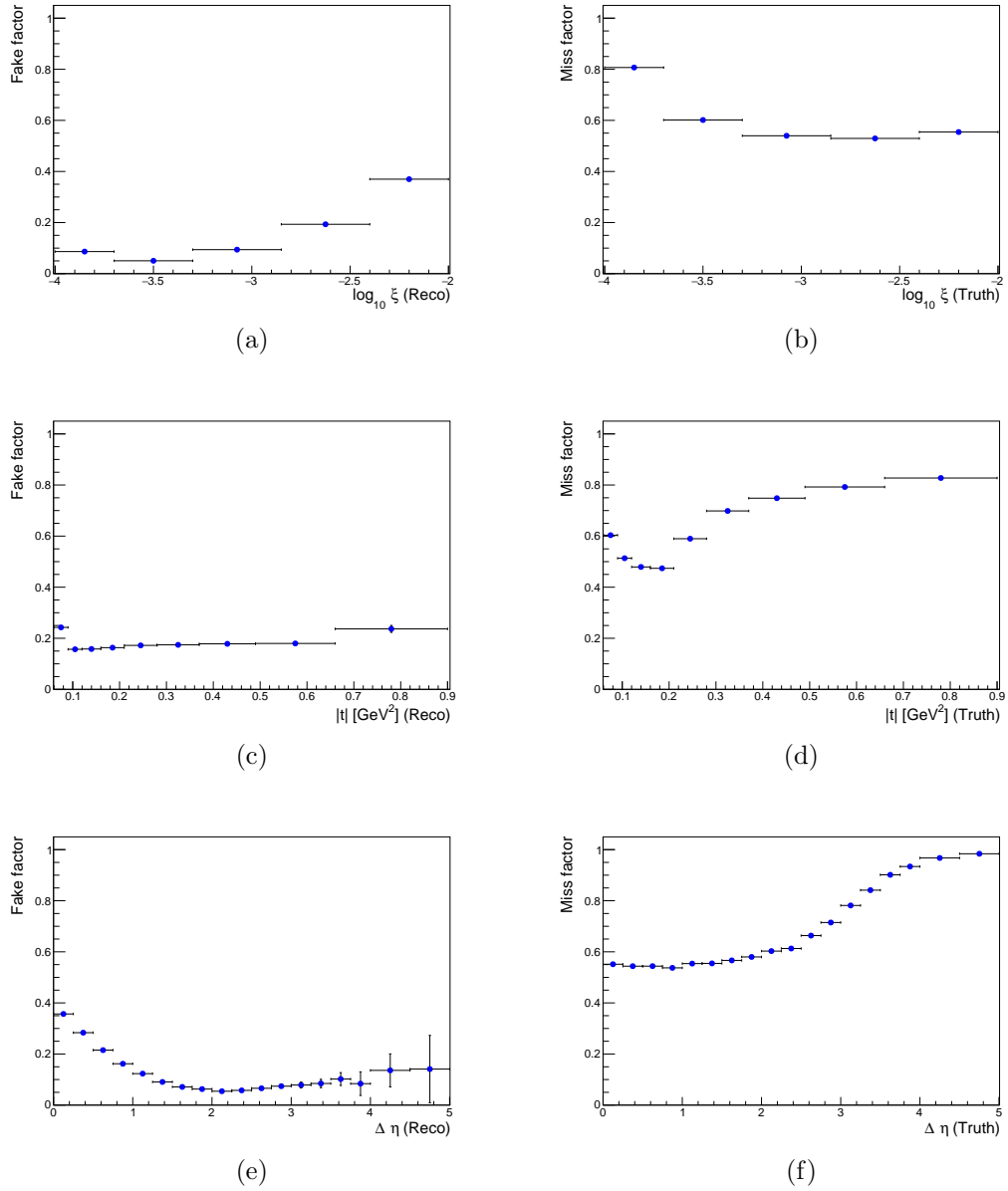
Figure 7.2: The fake and miss factors, defined in equations 7.4 and 7.5, respectively.
