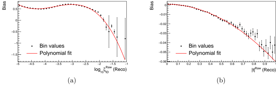
Figure 4.12: The bias plotted as a function of the reconstructed variable. The raw, uncalibrated values are shown as black points and the fitted polynomials are shown as red curves.
