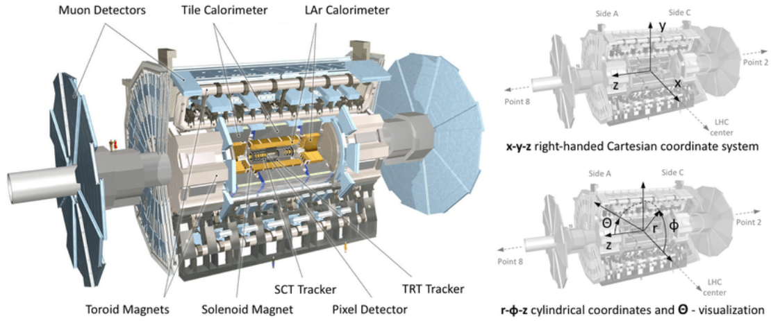
Figure 3.2: The major components of ATLAS detector and the coordinate systems used[95].
