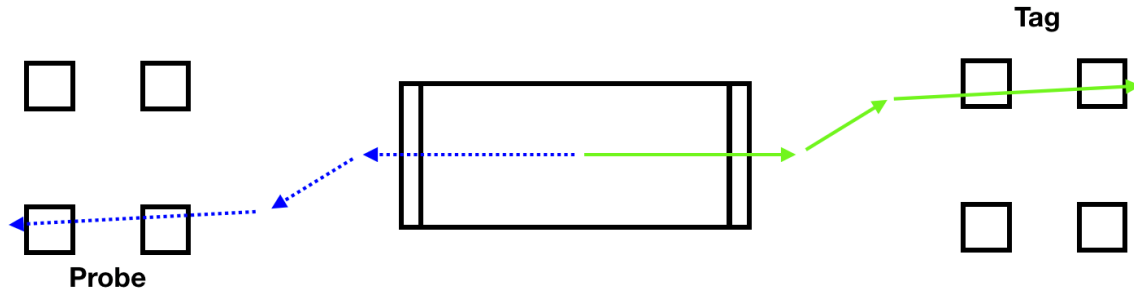
Figure 5.6: The tag and probe method. The solid green lines indicate the tag arm, which is required to contain a track passing the offline selection. The diagonally opposite arm is then probed for a corresponding proton, assuming elastic scattering, as indicated by the dashed blue line.
