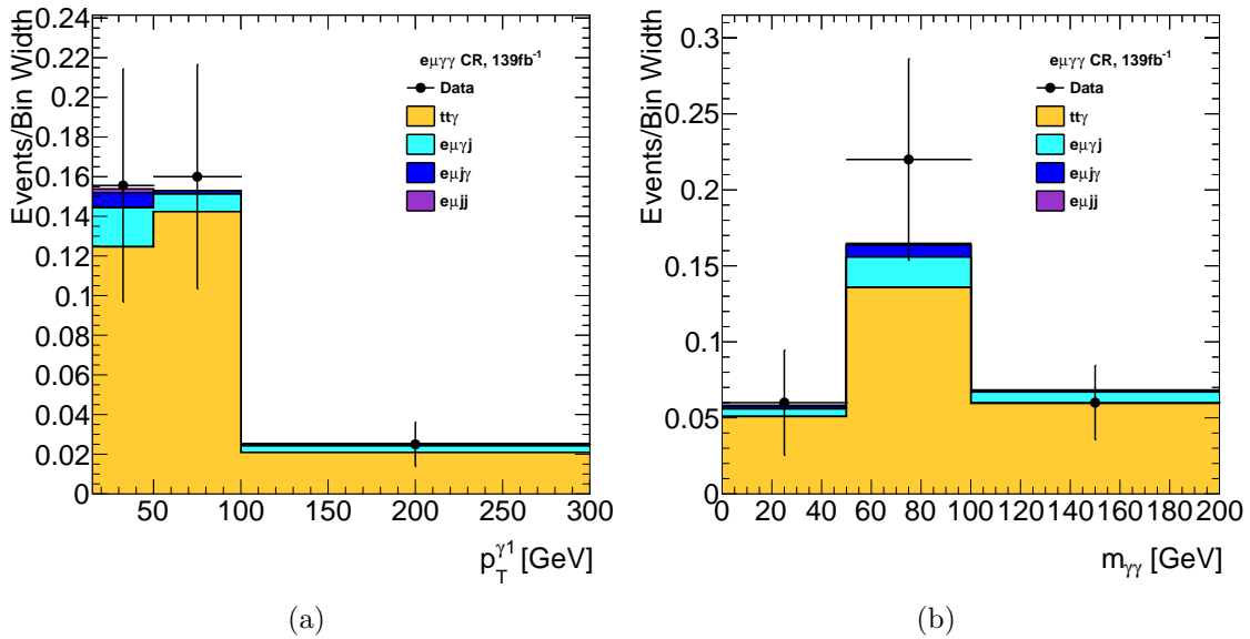
Figure 6.4: The comparison of prediction to data in the e\mu\gamma\gamma control region as a function of (a) leading photon p_T and (b) diphoton invariant mass.
