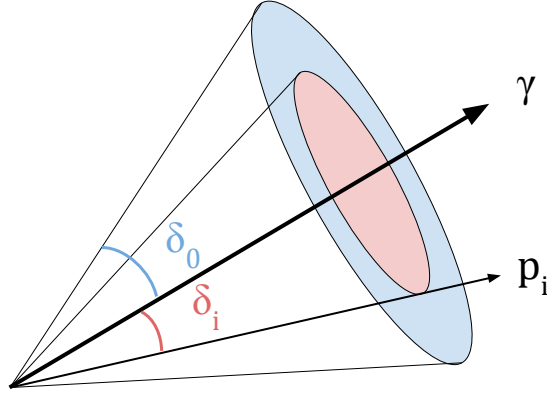
Figure 5.7: A diagram showing the angular separations considered in the Frixione isolation requirement. The angular separation between parton p_i and the photon ( \gamma ) is given as \delta_i and all partons with \delta_i < \delta_0 are considered.
