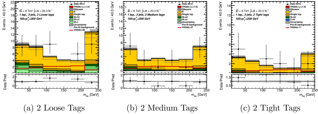
Figure 10.5: Postfit distributions of dijet invariant mass, m_{bb} , in the cut-based E_T^{\text{miss}} triggered 3-jet p_T(W) = 160 - 200 GeV regions. The format is the same as Figure 10.1.
