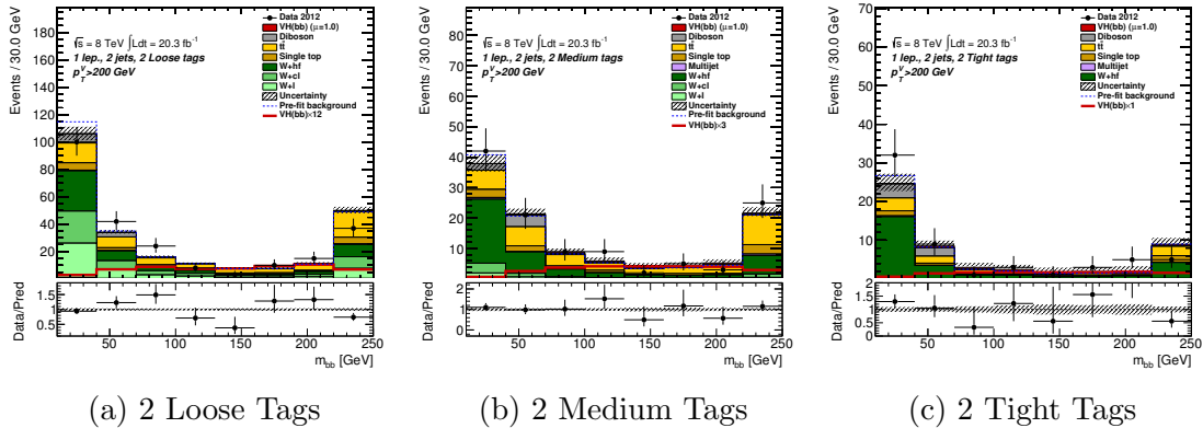
Figure D.5: Positfit distributions of dijet invariant mass, m_{bb} , in the cut-based combined 2-jet p_T(W) > 200 GeV regions. The format is the same as Figure D.1.
