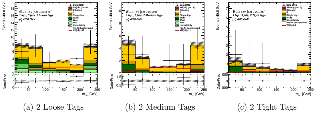
Figure 10.6: Postfit distributions of dijet invariant mass, m_{bb} , in the cut-based E_T^{\text{miss}} triggered 3-jet p_T(W) > 200 GeV regions. The format is the same as Figure 10.1.
