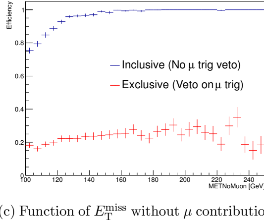
Figure 7.2: E_T^{\text{miss}} trigger efficiency for the WH \rightarrow \ell\nu b\bar{b} Signal Monte Carlo at a Higgs mass m_H=125 GeV. The efficiency is shown as a function of p_T(\mu) , E_T^{\text{miss}} (MET) and E_T^{\text{miss}} without the muon contributions counted (METNoMuon). The efficiency is shown both inclusively and exclusively, with a veto on the muon triggers used in the Nominal analysis. A preselection of exactly one signal muon, 2 loose jets has been applied.
