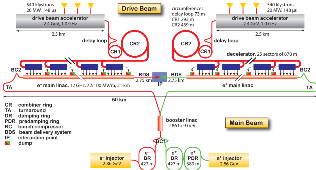
Figure 2.4: The CLIC Collider. Layout for the CLIC accelerator at 3 TeV. For the lowest energy stage there will only be one drive beam constructed which will power both main beams[22]
