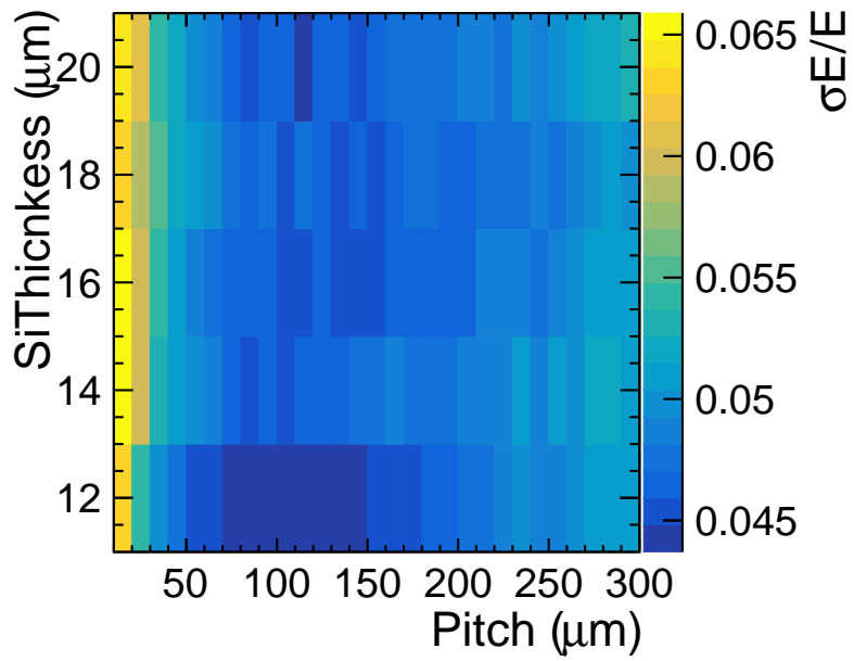
Figure 6.14: Energy resolution for 50 GeV photons.
