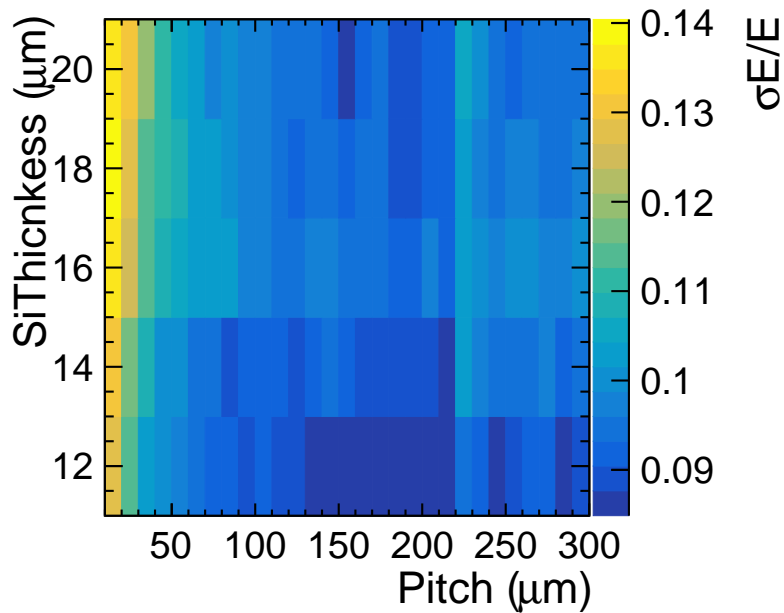
Figure 6.26: Energy resolution for 10 GeV photons after DigiMAPS is applied but without clustering.
