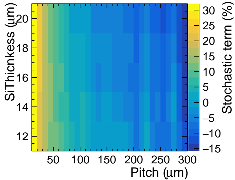
Figure 6.20: Stochastic term of the energy resolution fits for all pixel configurations when including clustering, noise, dead space and threshold spread.
