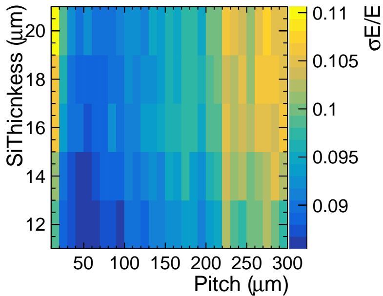
Figure 6.23: Energy resolution for 10 GeV photons after DigiMAPS is applied.
