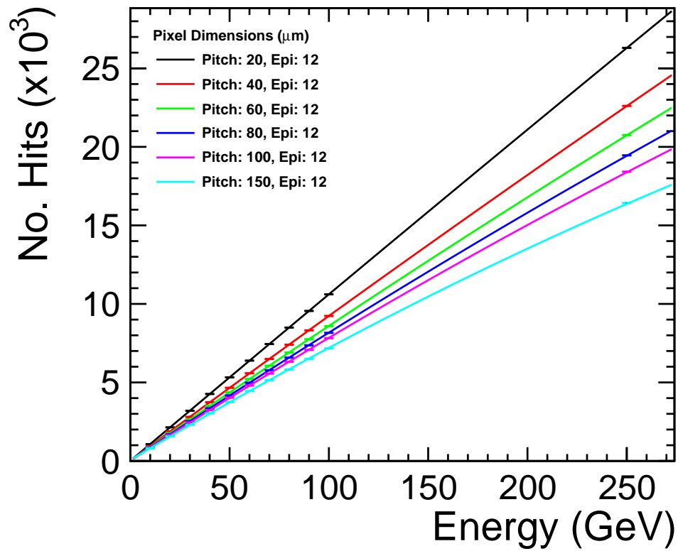
Figure 6.5: Calibration curves describing the relationship between the number of pixel hits observed and the energy of the incident particle for various pixel configurations.
