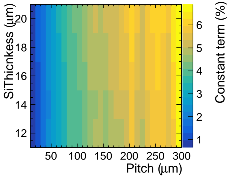
Figure 6.22: Constant term of the energy resolution fits for all pixel configurations when including clustering, noise, dead space and threshold spread.
