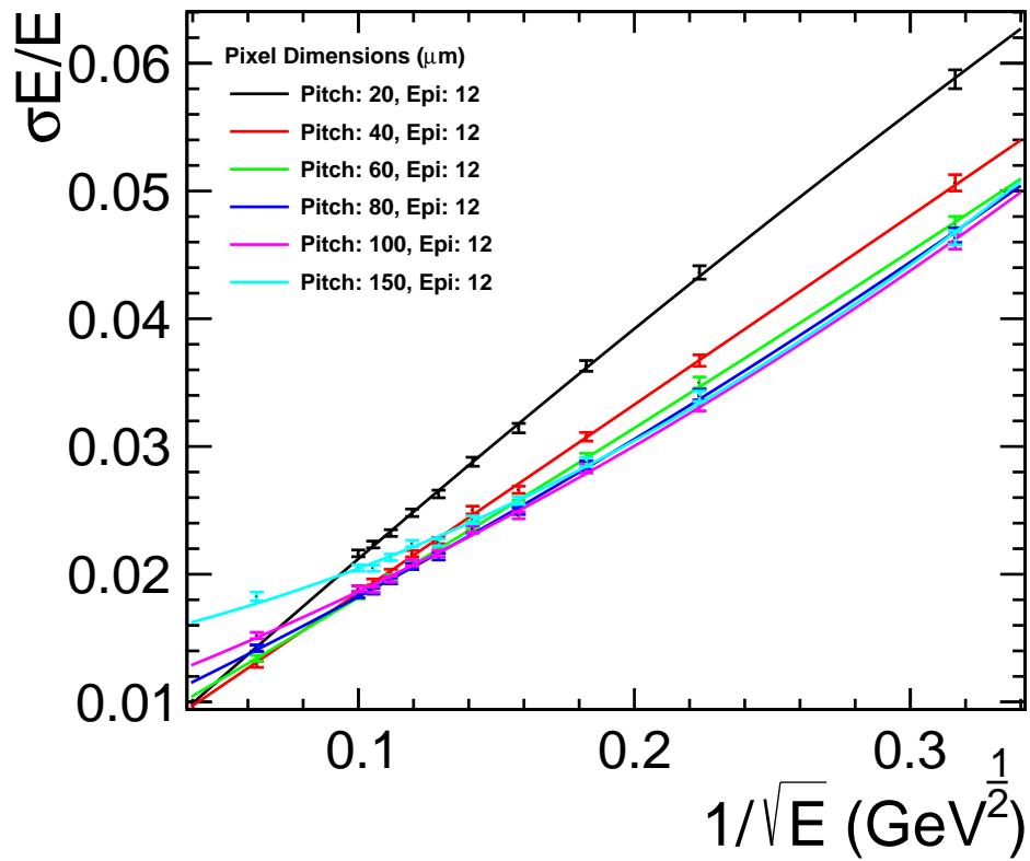
Figure 6.6: Energy resolution curves describing the variation of the energy resolution with the energy scale
