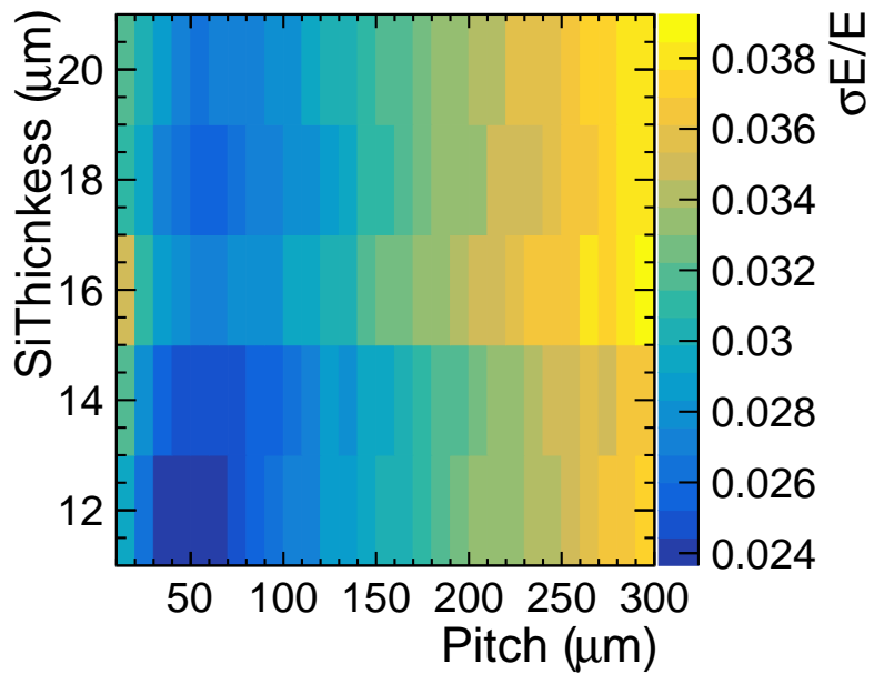
Figure 6.15: Energy resolution for 250 GeV photons.
