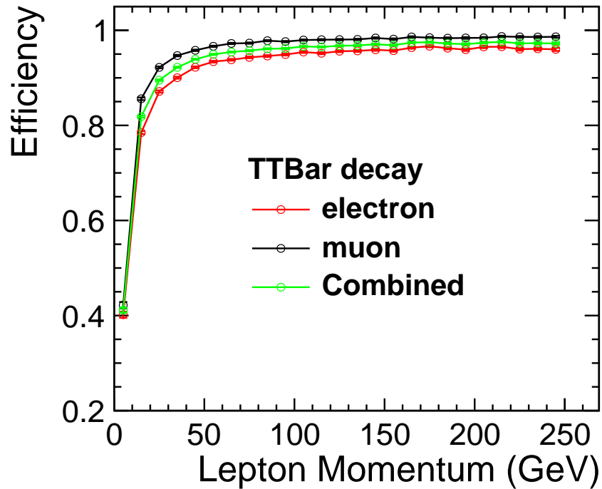
Figure 5.6: Efficiency for finding the isolated lepton as a function of the leptons momentum.
