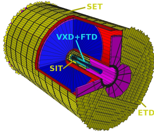
Figure 2.8: Silicon Tracking Systems For ILD [28]
