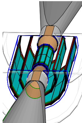
Figure 2.7: Proposed vertex detector geometry for ILD [28]
