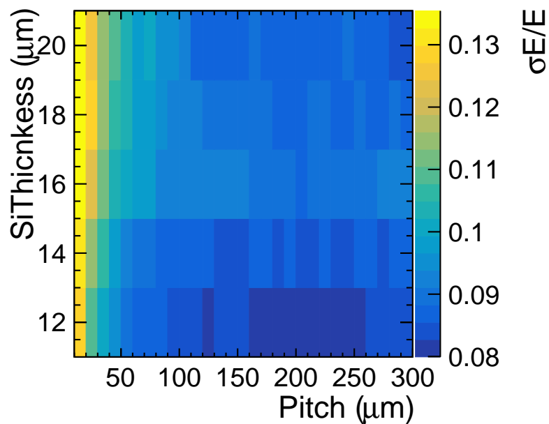
Figure 6.13: Energy resolution for 10 GeV photons.
