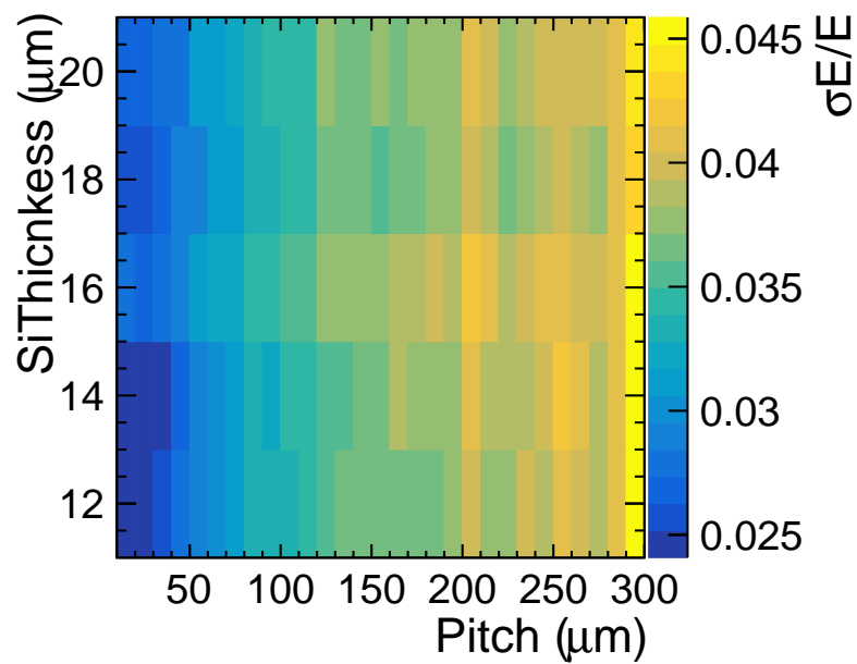
Figure 6.25: Energy resolution for 250 GeV photons after DigiMAPS is applied.
