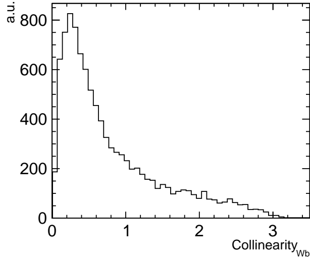
Figure 5.9: Collinearity of W and b jets from top decays. The pair are typically too collimated to allow the b-jet and the pair of jets from the W decay to be successfully resolved into three distinct objects.
