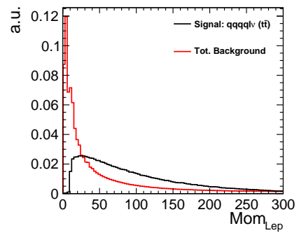
(n) Lepton momentum
