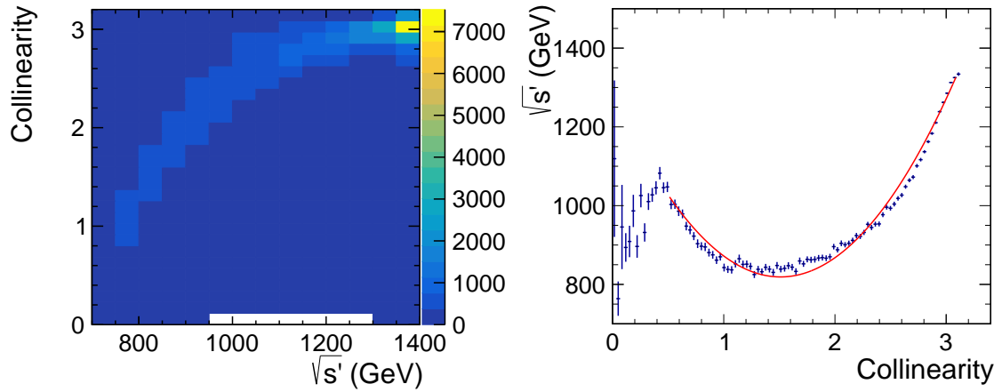
(a) Reconstructed collinearity of the t\bar{t} pair as a function of generator \sqrt{s'} . (b) Profiled generator \sqrt{s'} distribution as a function of reconstructed collinearity.
