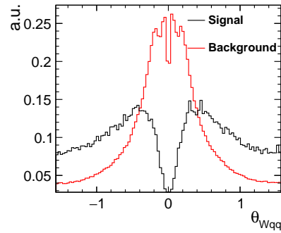
(b) Angle of W relative to beam axis
