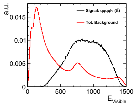
(b) Visible Energy
