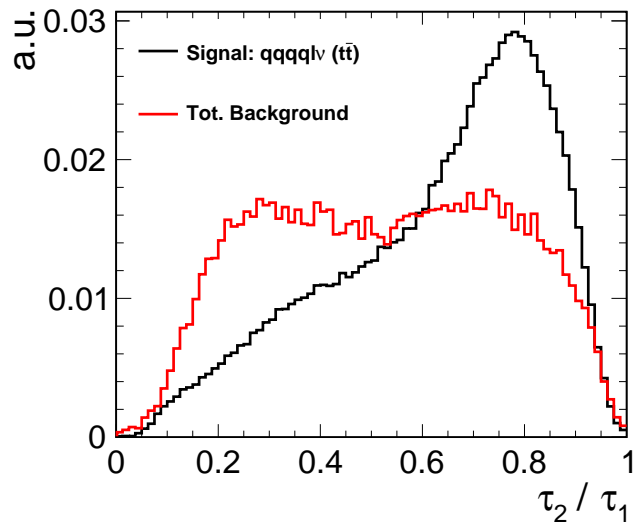
Figure 5.20: Ratio of \tau_2 to \tau_1 for the leptonic fat jet for both signal and background processes.
