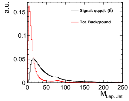
(f) Mass of leptonic fat jet
