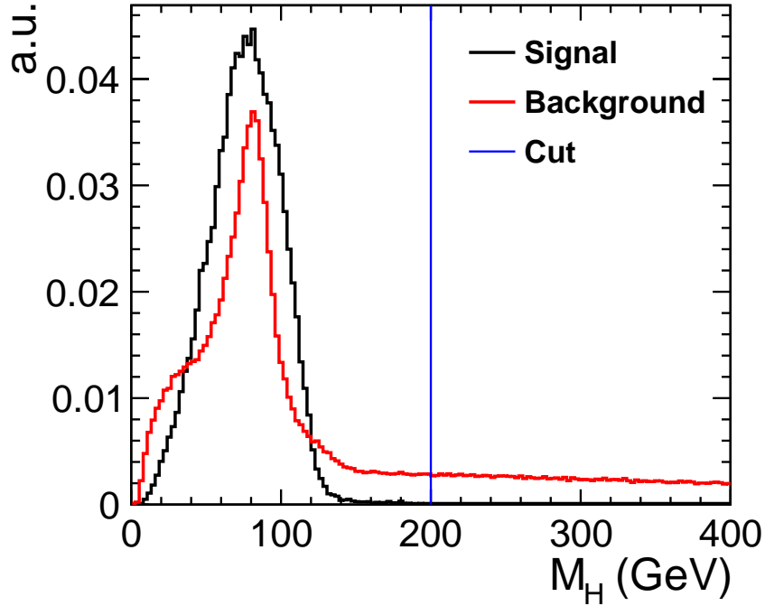
Figure 4.8: Mass of the reconstructed Higgs for the signal process and dominant backgrounds ( ee \rightarrow H\nu\nu (non-signal) and ee \rightarrow qql\nu ). Both signal and background are normalised to unity.
