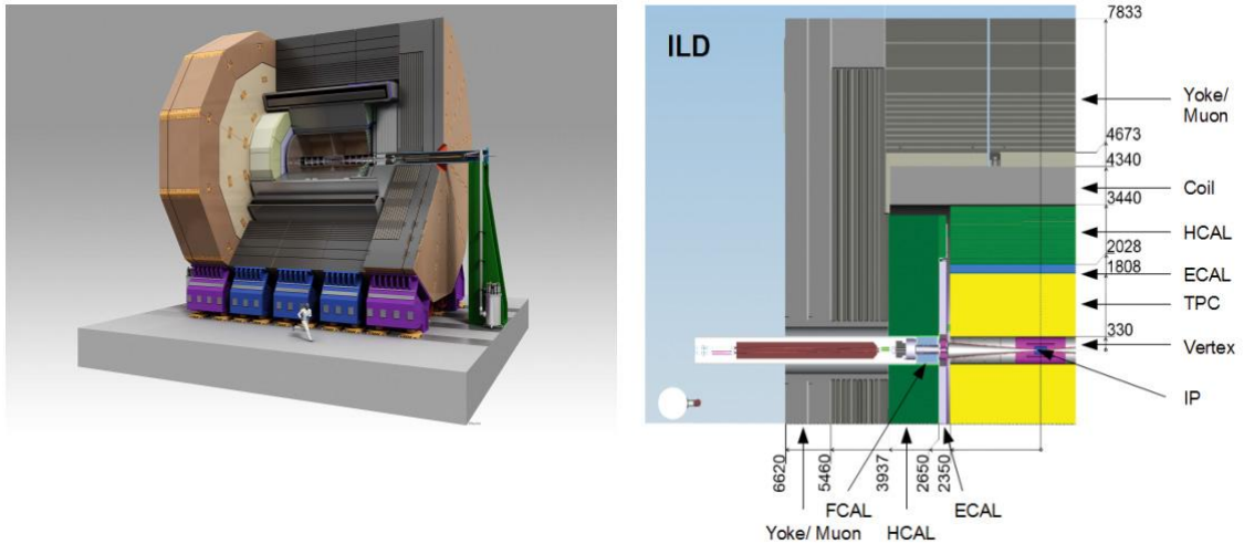
Figure 2.6: The International Large Detector Concept (left). Schematic of the ILD showing the key components in a one-quarter view of a vertical section of the detector (right). Dimensions are given in mm [16]. The z -axis is defined to be that parallel to the beam pipe, r is the radial distance from the beam and \theta is the polar angle measured relative to the z -axis.
