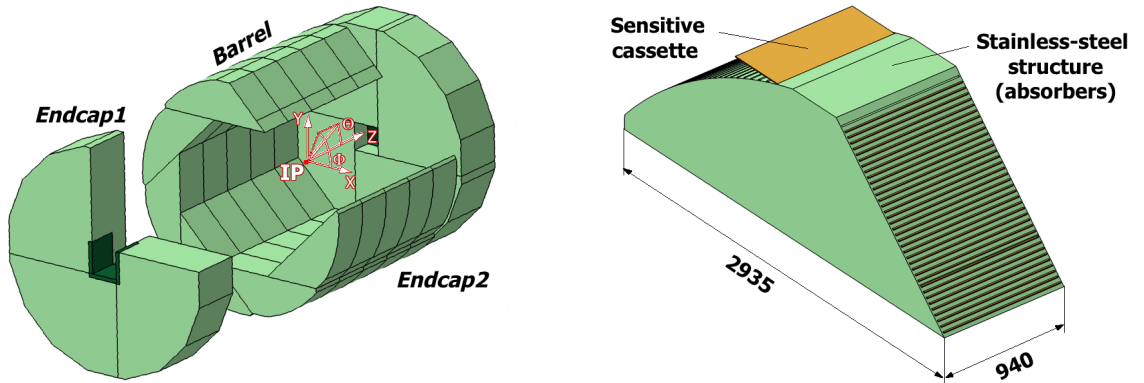
Figure 2.10: The Overall ILD HCAL Structure (left) and one individual module (right). The HCAL is made up 40 modules, each containing 30 detector slabs. The modules are combined into groups of 5 referred to as a stave which extend along the full length of the barrel. There are then 8 of these staves arranged in a circle to create the circumference of the barrel [28].
