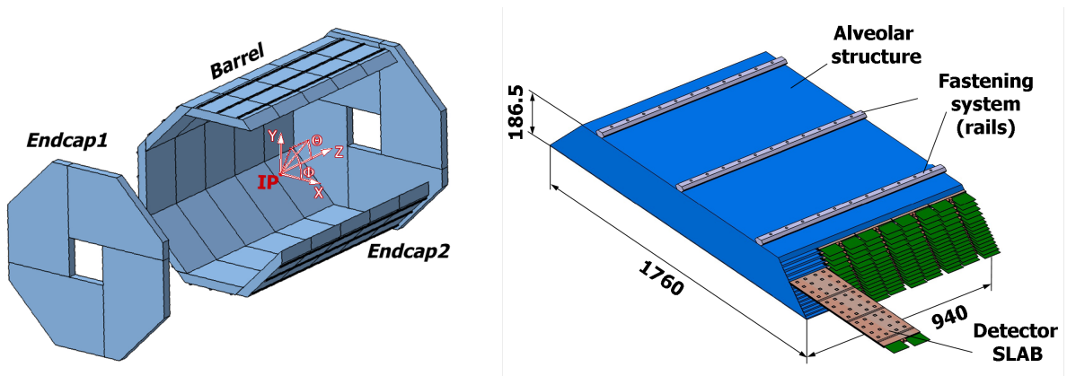
Figure 2.9: The Overall ILD Structure (left) and one individual module (right). The ECAL is made up 40 modules, each containing 30 detector slabs. The modules are combined into groups of 5 referred to as a stave which extend along the full length of the barrel. There are then 8 of these staves arranged in a circle to create the circumference of the barrel [28].
