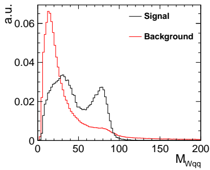
(m) Mass of hadronically decaying W
