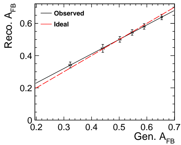
(b) 900-1200 GeV
