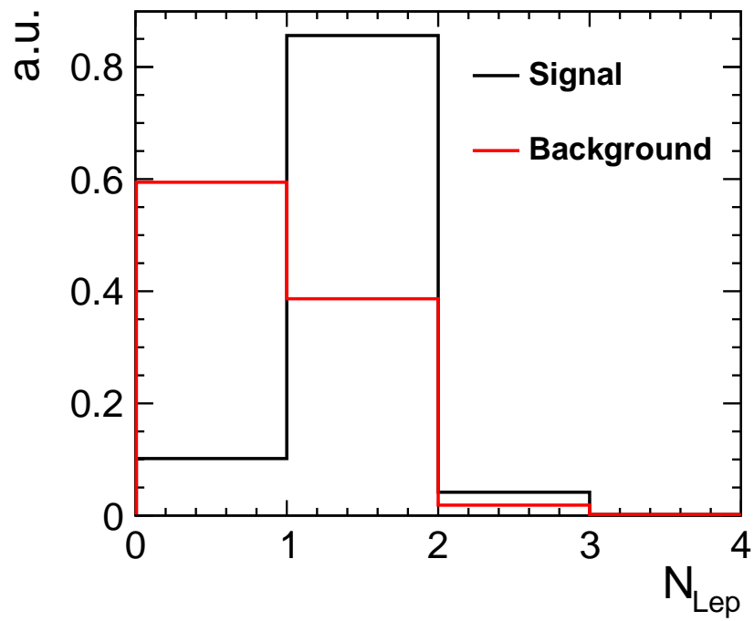
Figure 4.10: Number of loose selected leptons for the signal process and dominant backgrounds ( ee \rightarrow H\nu\nu (non-signal) and ee \rightarrow qql\nu ). Both signal and background are normalised to unity.
