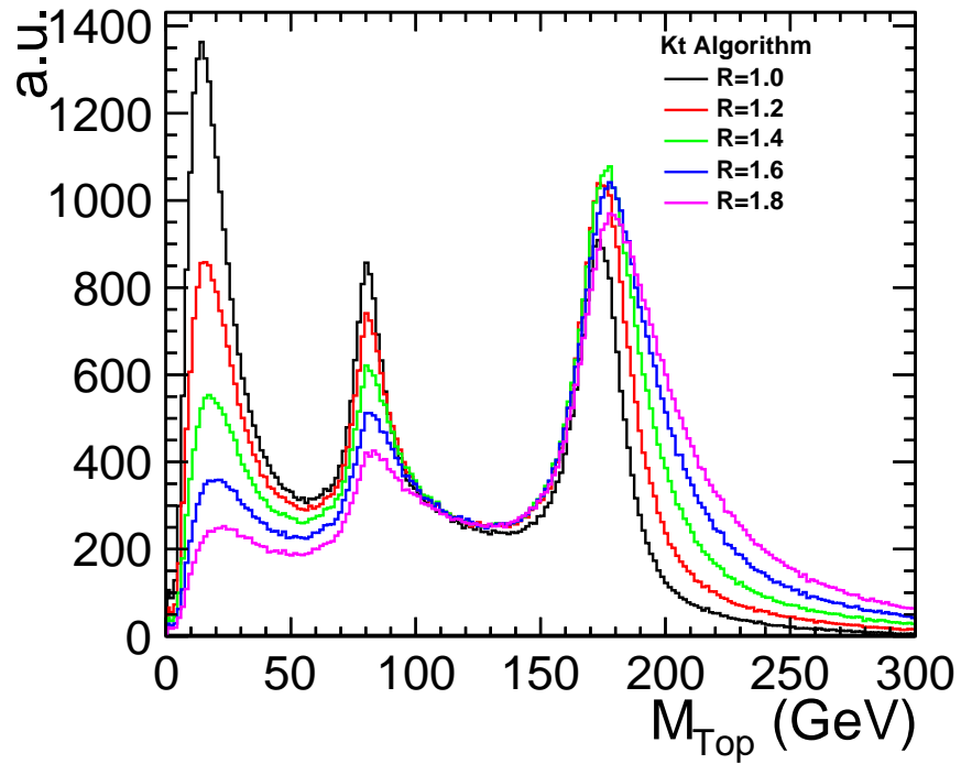
(a) kt algorithm
