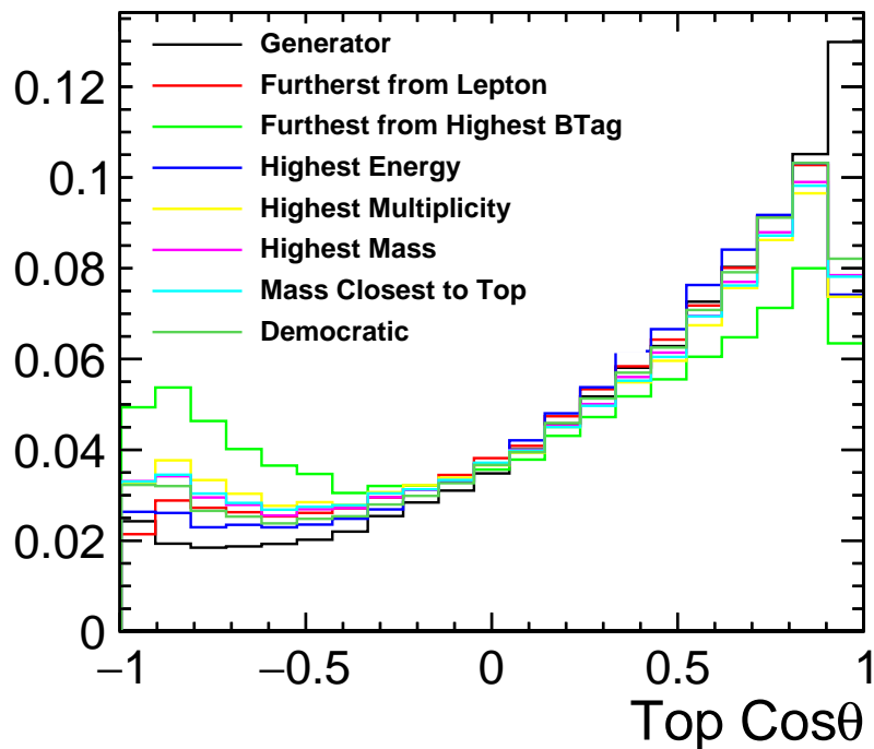
Figure 5.16: Reconstructed \cos\theta distribution for various jet association methods. The expected distribution from truth level information is included for reference.
