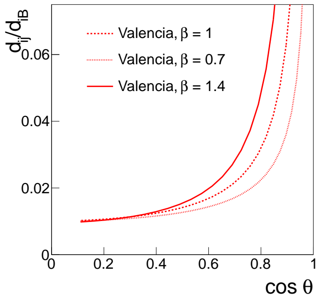
Figure 5.10: Effect of the Valencia \beta parameter on d_{ij}/d_{iB} for a pair of particles produced at a fixed energy and angular separation as a function of their polar angle[62].
