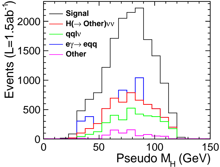
Figure 4.16: Stacked pseudo Higgs mass distributions following event selection for the nominal integrated luminosity of 1.5 \text{ ab}^{-1} . The effect of limited events in the e\gamma samples is clearly visible.
