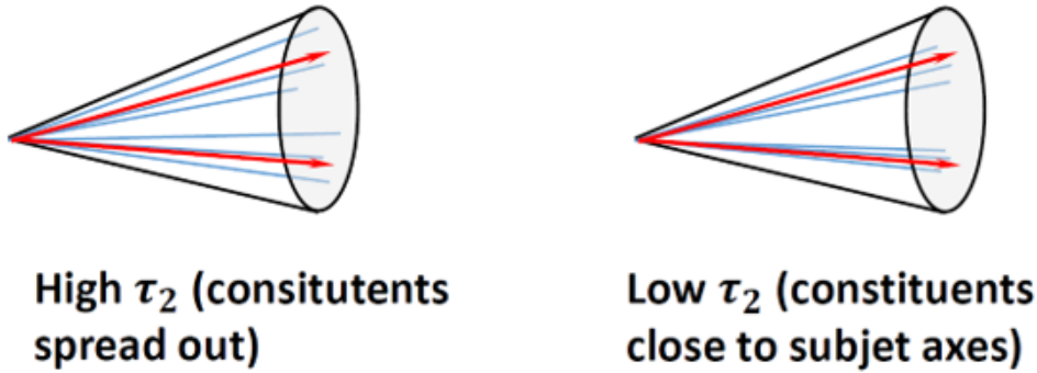
Figure 5.19: Diagrammatic representation of N-subjettiness.
