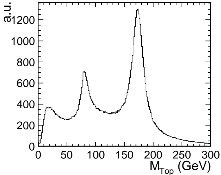
Figure 5.12: Reconstructed top mass for the Valencia algorithm ( R=1.5 , \beta=1 , \gamma=1 ) in events close to the nominal collision energy ( E > 1.2 TeV).
