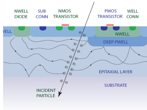
Figure 6.2: CMOS MAPS sensor including deep p well implant to prevent parasitic losses to the PMOS transistor[70]
