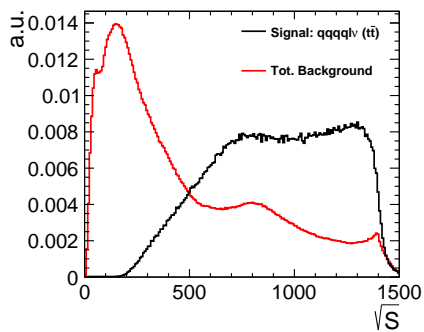
(a) Centre-of-mass
