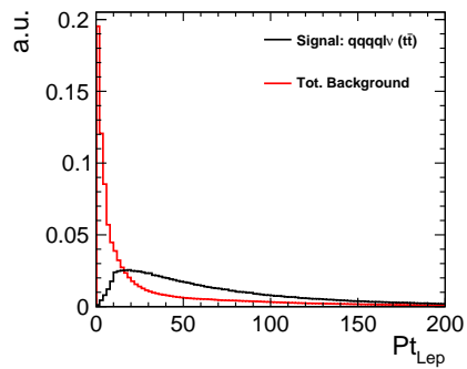
(m) Lepton transverse momentum
