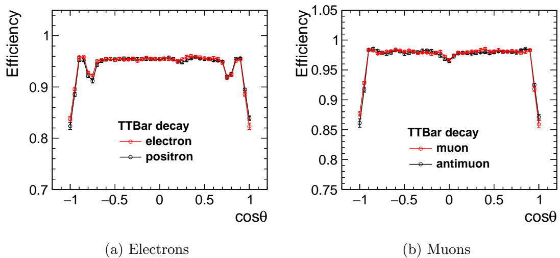
Figure 5.8: Charge tagging efficiency after 20 GeV lepton momentum cut. The efficiency is seen to be symmetric for leptons with momentum > 20 GeV.
