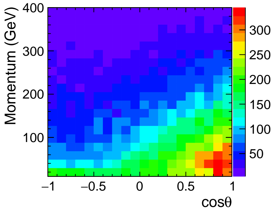
Figure 5.5: Correlation between lepton momentum and angle for positrons only.
