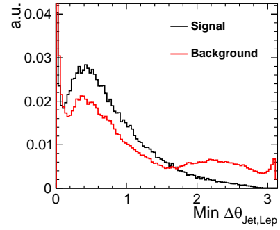
(h) Angular separation between lepton and nearest jet
