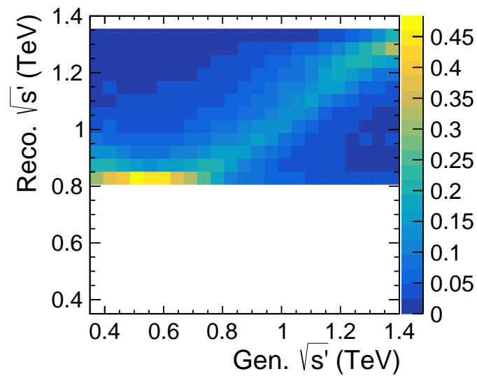
Figure 5.29: Reconstructed \sqrt{s'} vs generator \sqrt{s'} for collinearity method.
