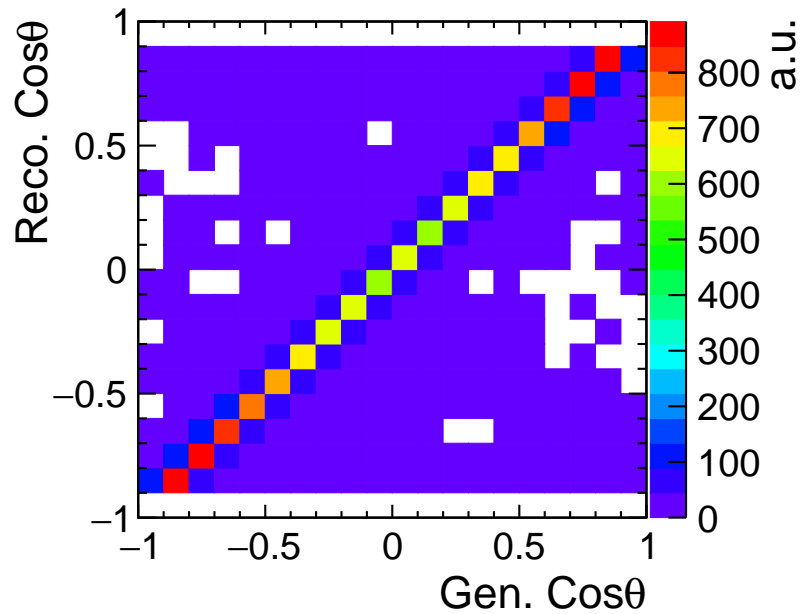
Figure 5.41: Correlation between \cos\theta reco. vs gen. after quality cuts are applied.
