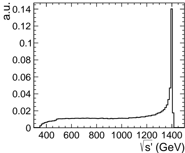
Figure 5.23: Expected \sqrt{s'} spectrum for t\bar{t} at 1.4 TeV.
