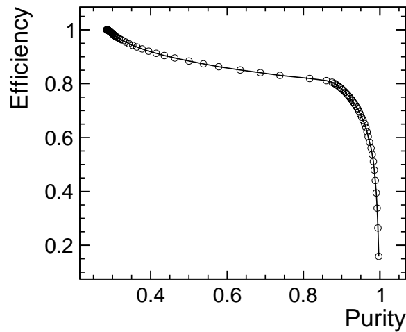
Figure 5.31: Purity vs efficiency for identifying b-jets, obtained from a sample of Z \rightarrow light, c and b quark events simulated at \sqrt{s} = 1.4 TeV.
