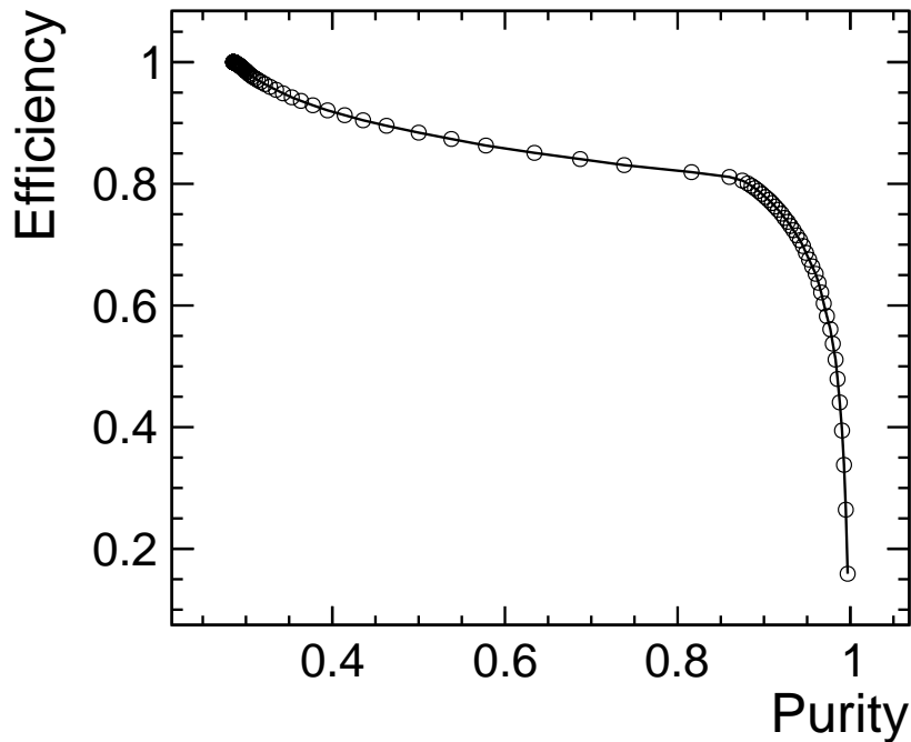
Figure 4.7: Purity vs efficiency for identifying b-jets, obtained from a sample of Z \rightarrow light, c and b quark events simulated at \sqrt{s} = 1.4 \text{ TeV} .
