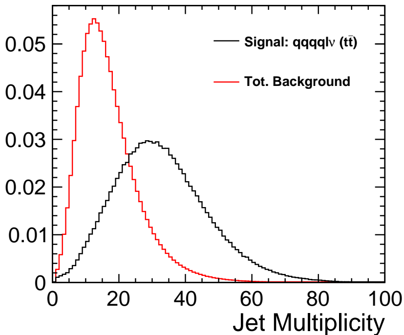
Figure 5.22: Jet multiplicity of the hadronic fat jet.
