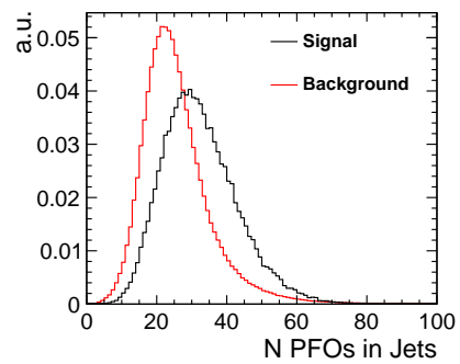
(p) nPFOs assigned to jets
