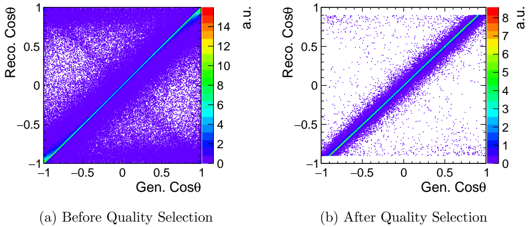
Figure 5.35: Effect of quality selection on agreement of \cos\theta reco. vs gen.
