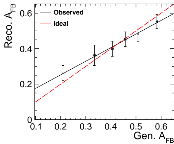
(c) 400-900 GeV
