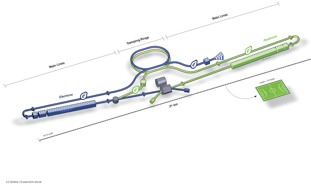
Figure 2.1: The ILC Collider[16]
