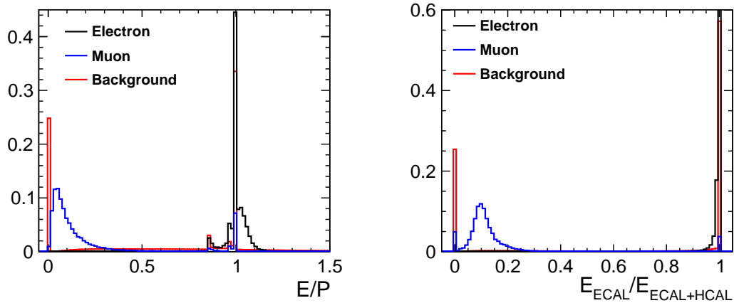
(a) Ratio of the sum of the energy deposited in ECAL and HCAL to the momentum of the charged particle. (b) Ratio of the energy deposited in the ECAL to the total energy deposited in the calorimeters.
