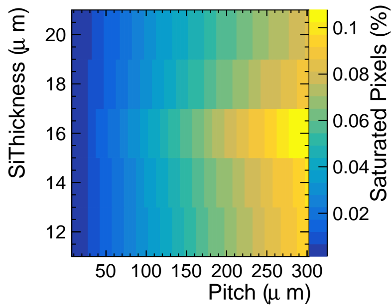
Figure 6.10: Percentage of pixels containing multiple hits as a function of the pixel dimensions for 100 GeV photons.
