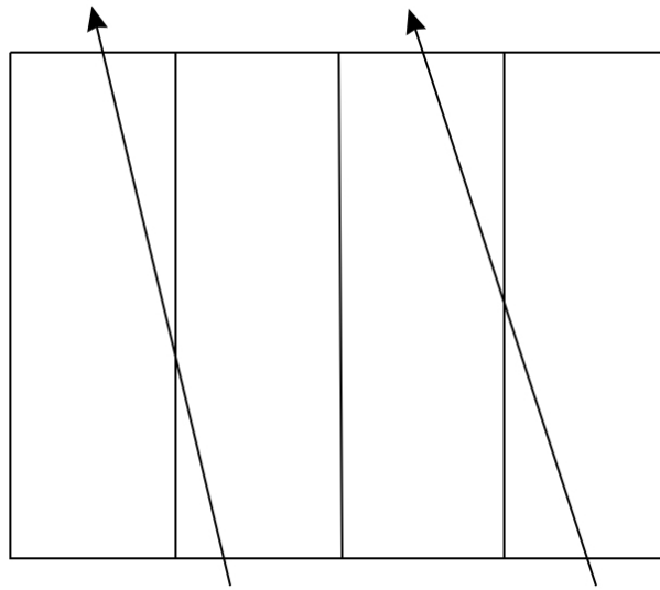
Figure 6.18: Aspect ratio is too high so particles penetrate multiple pixels per layer causing overcounting.
