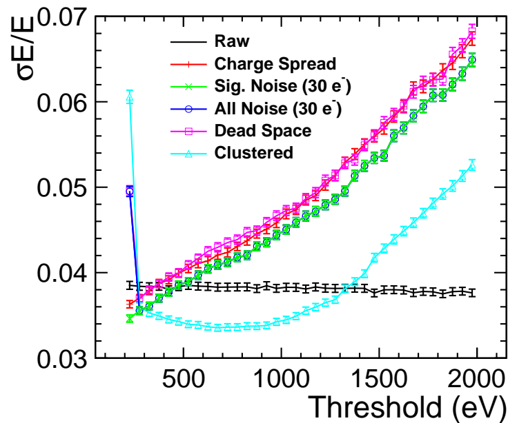
Figure 6.19: Variation in the energy resolution as a function of the threshold applied after each DigiMAPS effect is added. The effects are added sequentially in the order displayed in the legend.
