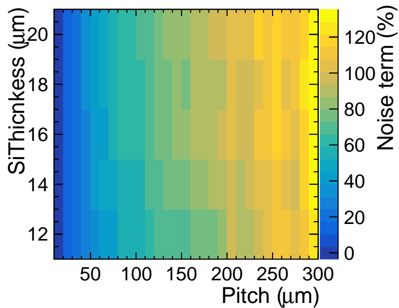
Figure 6.21: Noise term of the energy resolution fits for all pixel configurations when including clustering, noise, dead space and threshold spread.
