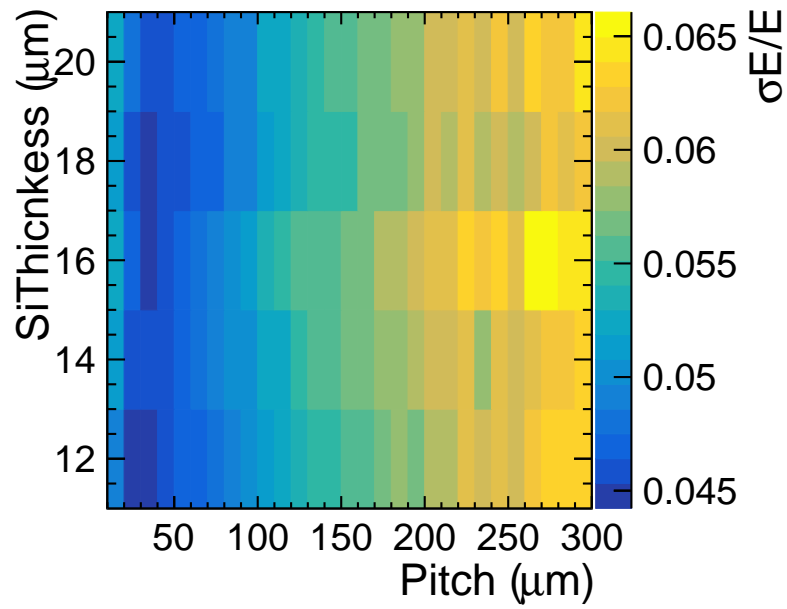
Figure 6.24: Energy resolution for 50 GeV photons after DigiMAPS is applied.
