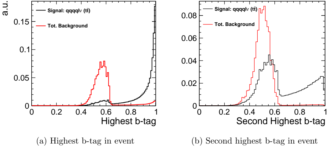
Figure 5.32: B-Tagging performance.
