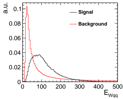
(c) Energy of hadronically decaying W
