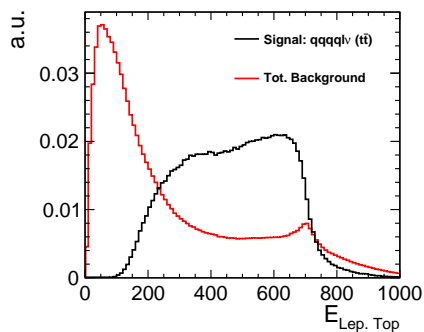
(s) Energy of the leptonically decaying top
