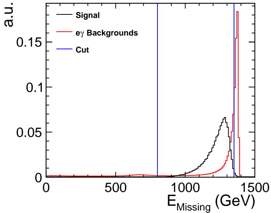
Figure 4.12: Missing energy for the signal process and e\gamma backgrounds. Both signal and background are normalised to unity.
