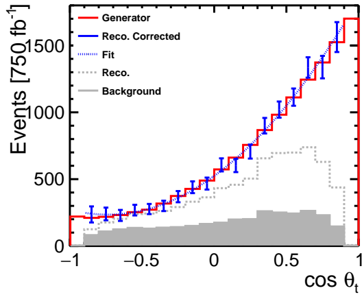
(a) High energy, -80% polarization
