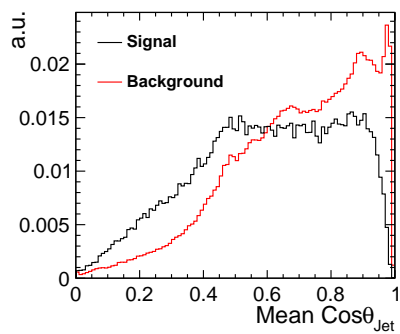
(e) Average \cos\theta of jets
