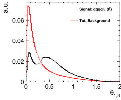
(i) \theta_{1,3}
