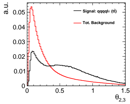
(k) \theta_{2,3}
