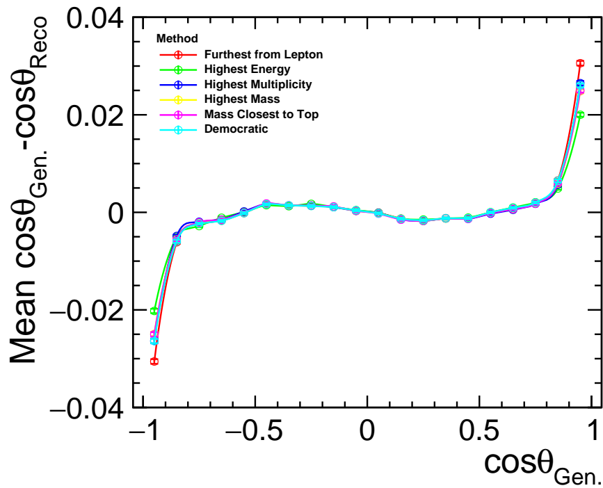
(a) Mean
