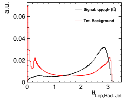
(o) Number of lepton candidates with E > 30 (p) Angular separation of the lepton and hadronic fat jet
