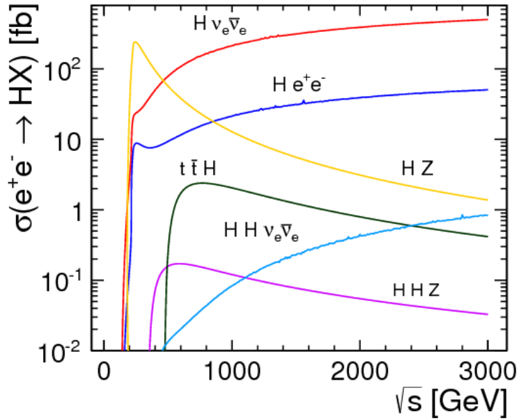
Figure 4.1: Cross sections for dominant Higgs production mechanisms as a function of energy [1]. Higgs production via WW -fusion is shown in red.
