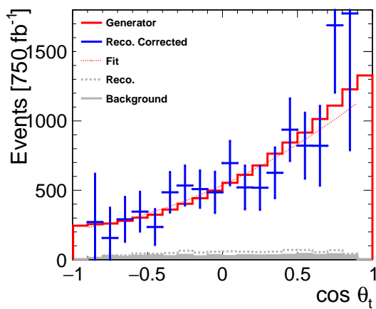
(e) Low energy, -80% polarization
