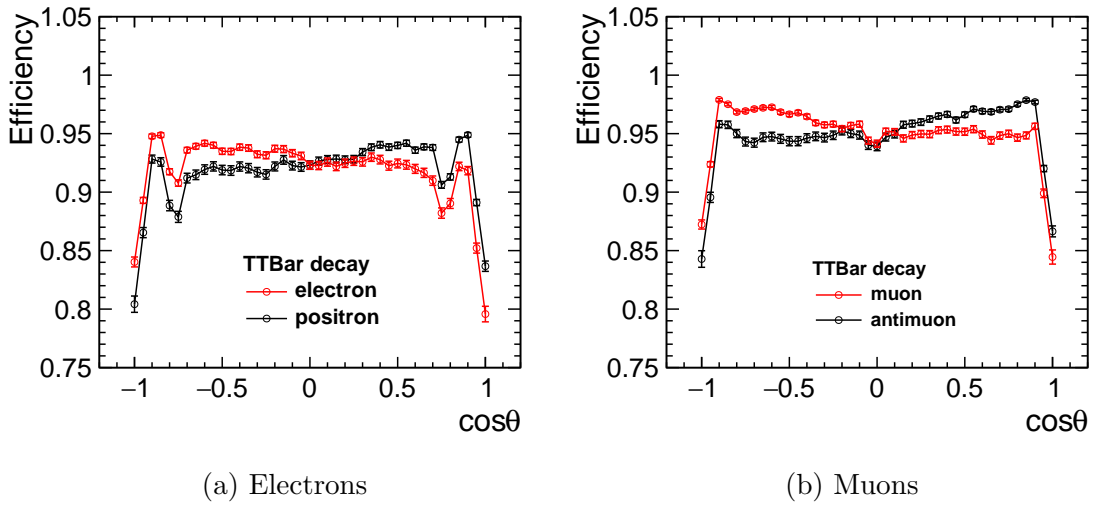
Figure 5.4: Angular dependence of lepton finding for particles vs antiparticles.
