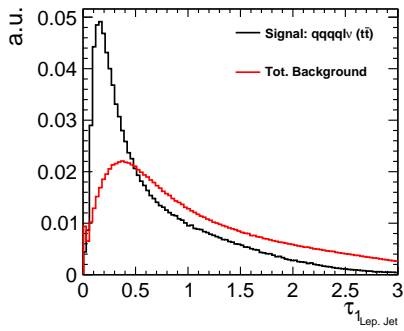
(g) Leptonic fat jet \tau_1
