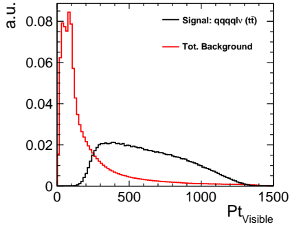
(c) Visible Transverse Momentum
