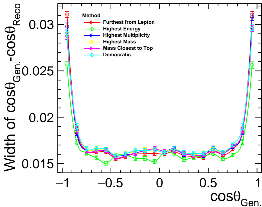
(b) Width
