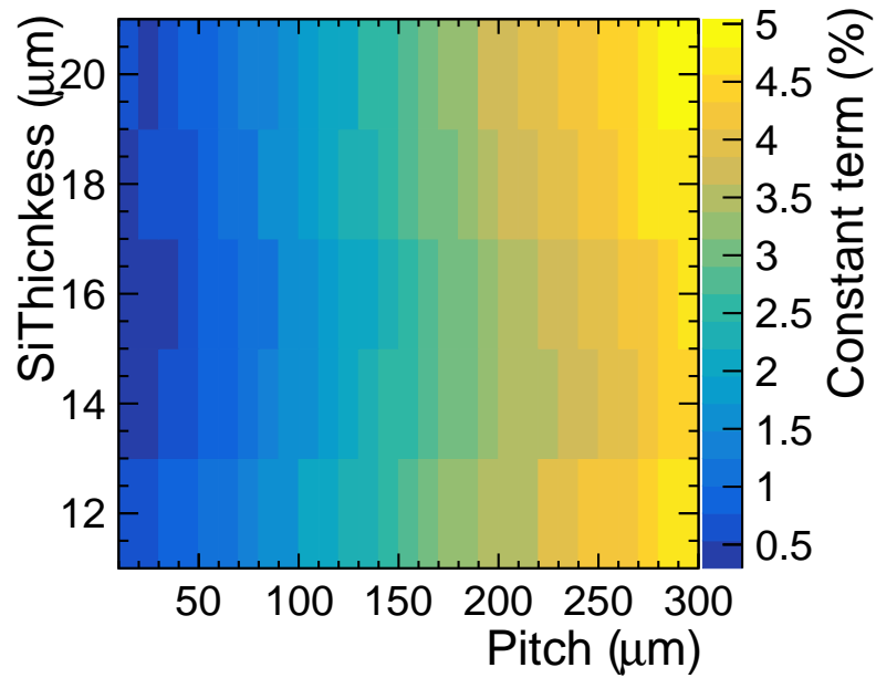
Figure 6.9: Constant term of the energy resolution fits for all pixel configurations
