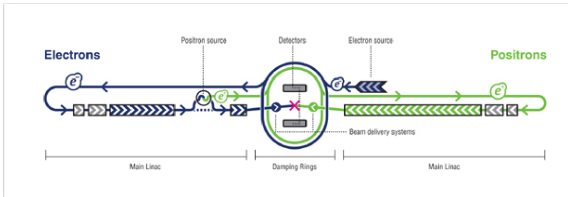
Figure 2.2: A simplified schematic of the ILC[16]
