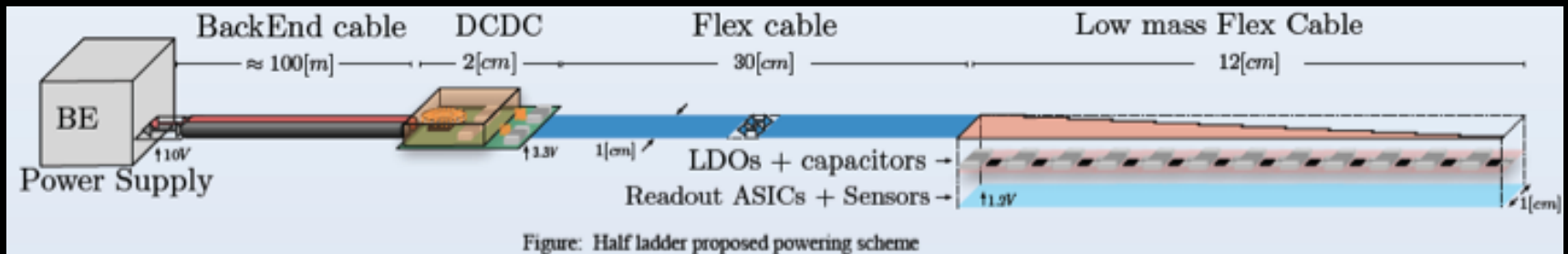
Figure: Half ladder proposed powering scheme
