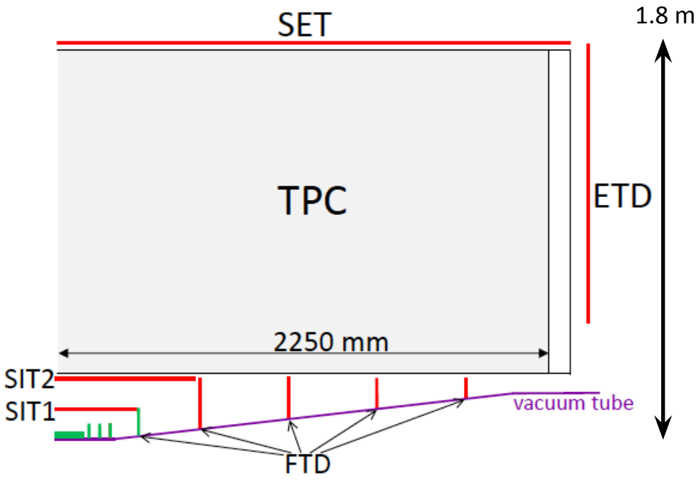
Time Projection Chamber (TPC) with MPGD readout
