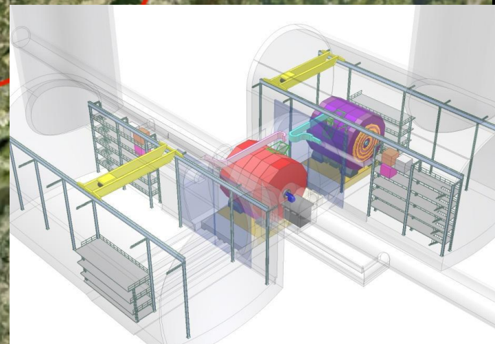
Central MDI & Interaction Region
